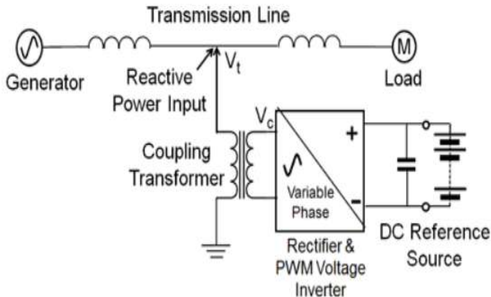
Fig. 1. Synchronous voltage and power factor compensation with reactive power
